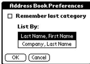
Address Book
